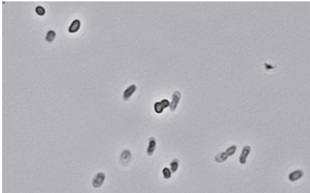
Fig. 2 Micrograph of a novel cultured greigite- and magnetite-producing bacterium, strain JCM 18010.
